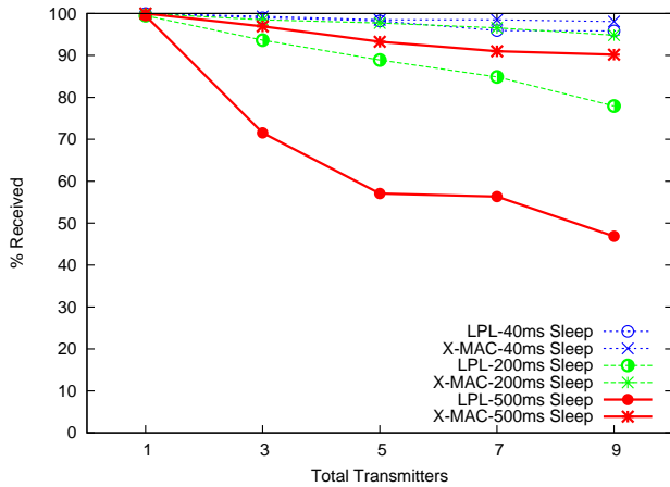
Figure 12. Reception success rate, 1 packet per second.
