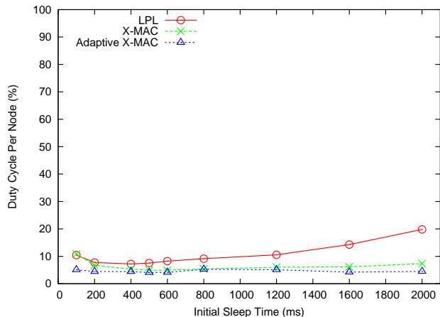
Figure 15. Average duty cycle of all nodes versus initial sleep times, 0.1 packet per second.
