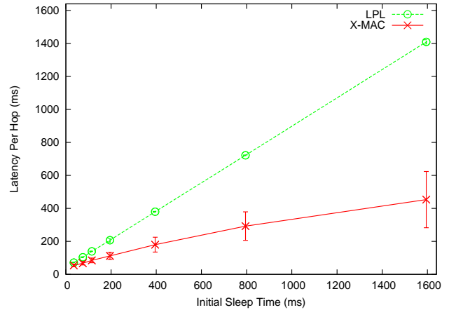
Figure 13. Latency per hop versus initial sleep times.
