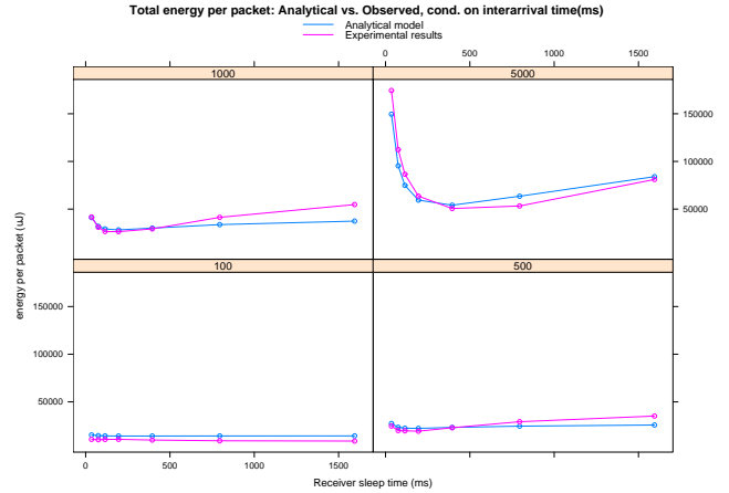
Figure 6. Comparison of analytic model and experimental results for total energy consumer per packet. Sub-figures are for different packet inter-arrival times.
