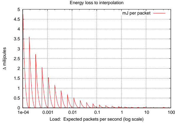
Figure 3. Energy waste per packet due to interpolation.
