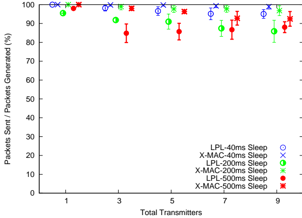
Figure 11. Fairness versus node density, 1 packet per second.
