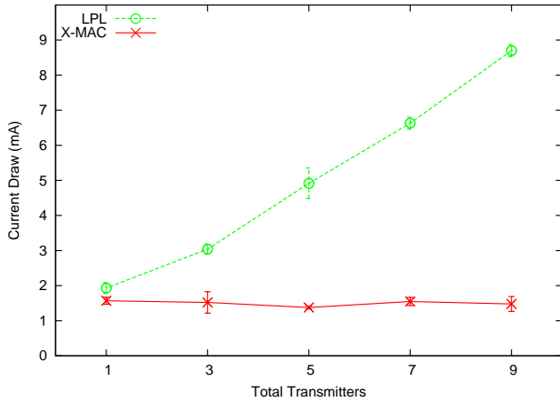
Figure 8. Power consumption per node versus density.
