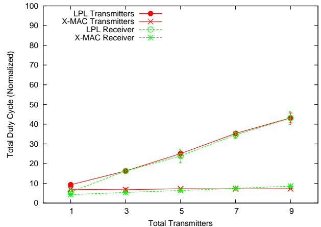
Figure 7. Duty cycles of non-contending senders and receiver and as a function of network density.
