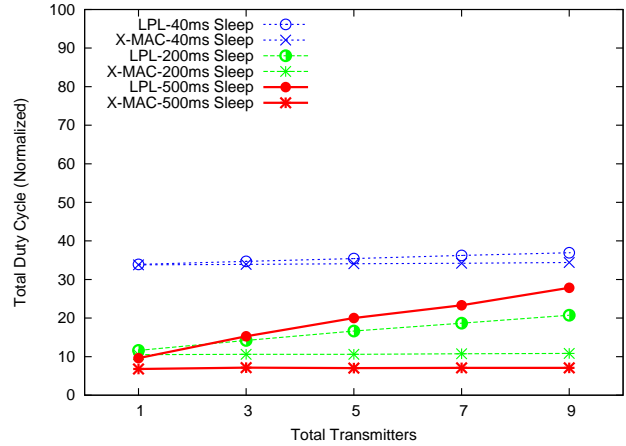
Figure 10. Duty cycle of contending senders, 1 packet per 10 seconds.
