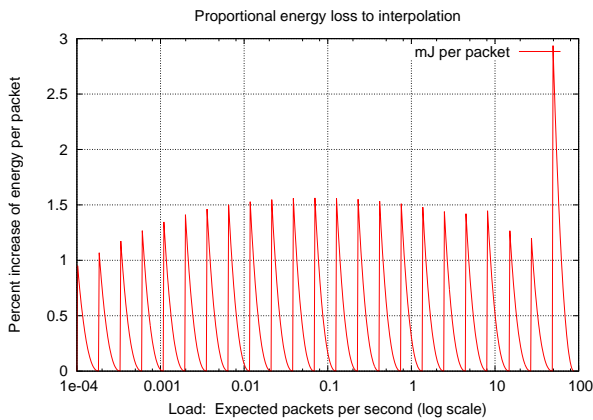
Figure 4. Energy waste as a fraction of optimum.
