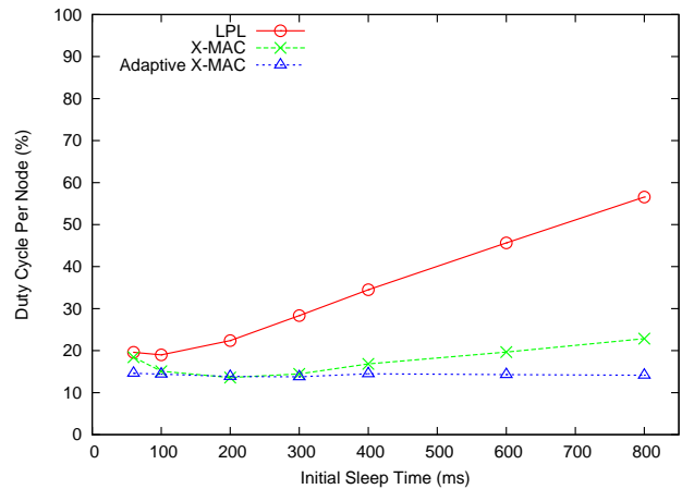
Figure 14. Average duty cycle of all nodes versus initial sleep times, 1 packet per second.
