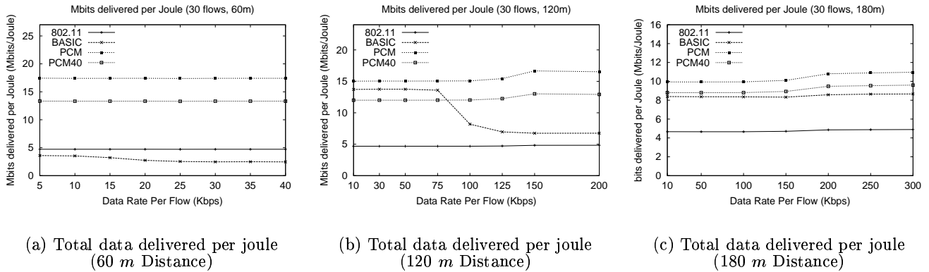
Figure 11: Chain topology: A large number of retransmissions in BASIC results in more energy consumption.
