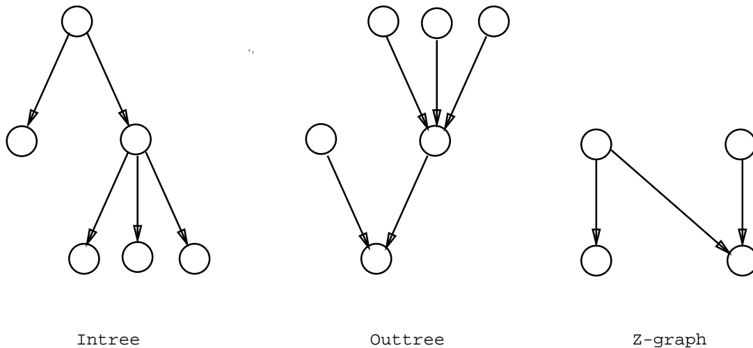
Figure 2: Precedence Relations
