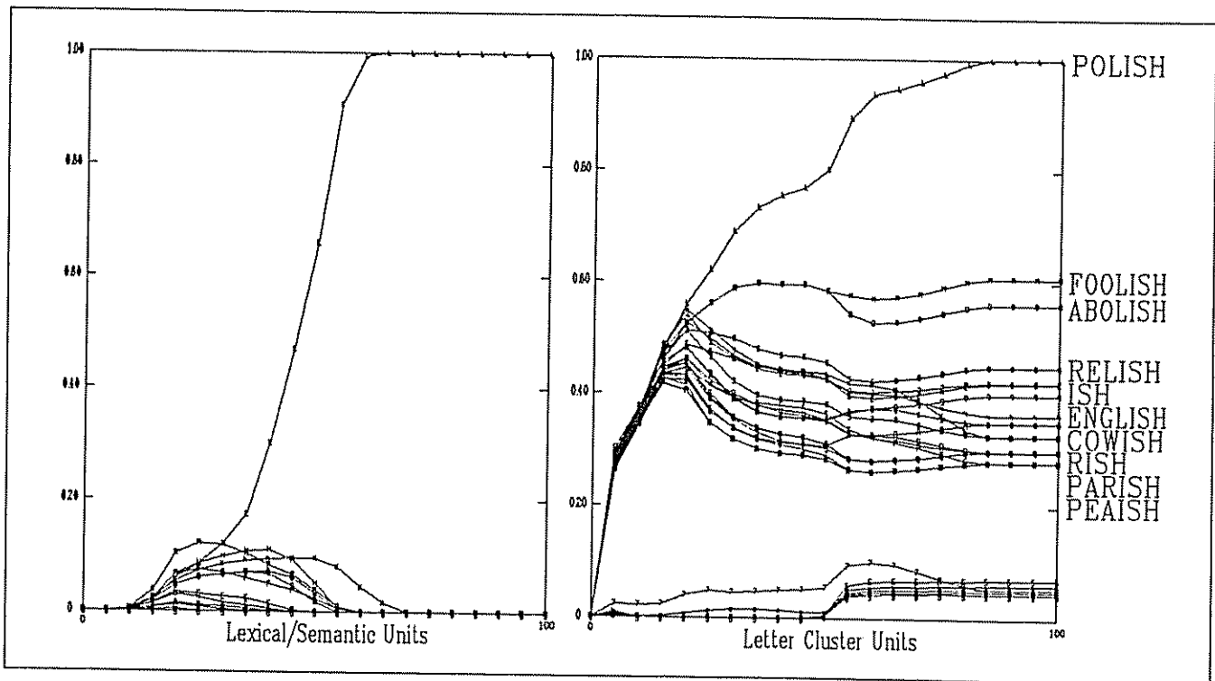
Figure 8. Activity in the PO net as a function of time for the stimulus PAUSH on a trial where the AM has selected the last three letters of the word. The PO net eventually reads out POLISH. The left graph summarizes activations of the semlex units over time, and the right graph activations of the letter cluster units. Each trace represents aggregate activity of a particular response and is labeled with a single digit or letter symbol. Traces corresponding to the same word in the two graphs use the same symbol. The 10 most active responses in the letter cluster graph are shown on the far right, roughly next to the corresponding trace. The aggregate semlex activity of a response is simply the average activity of its semlex units. The aggregate letter cluster activity of a response is a measure of the activity of the target clusters relative to nontarget clusters (see Appendix 4). Note that due to the distributed word representations, there will always be partial activity of response alternatives similar to the chosen one.
