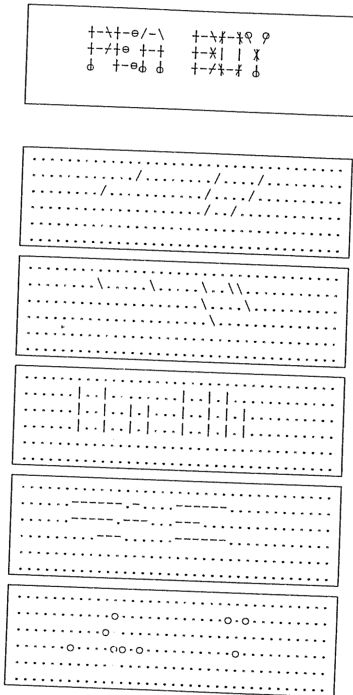
Figure 2. The top array shows the superimposed feature activations for a sample input PEA BOY, positioned on MORSEL's retina. The remaining arrays represent the individual feature maps. Each character in an array represents the activity of a single unit. A " " indicates that the unit is off, A, L, I, J, or V indicates activity of the corresponding unit in the 0°, 45°, 90°, 135° line segment map, respectively, and "o" indicates activity in the line segment terminator map.
