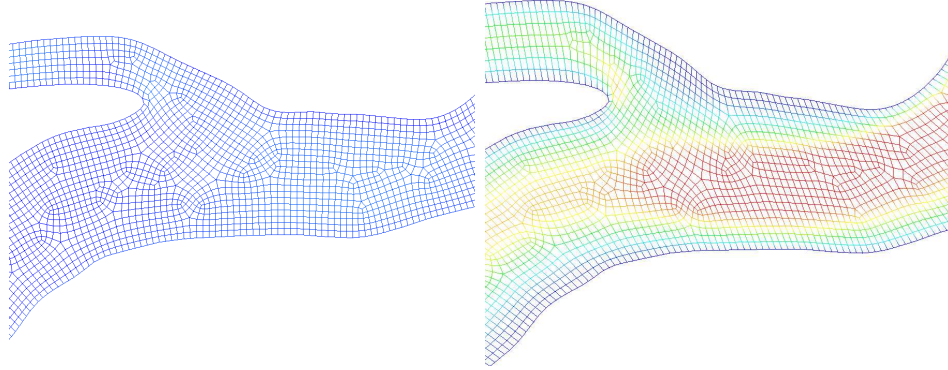
Figure 2: An undeformed fluid mesh in the reference configuration on the left, compared to the deformed mesh at systole on the right. This simulation is done with a low value of the Young's modulus E and a high inlet velocity to exaggerate the deformation of the fluid domain. The mesh conditioning remains quite acceptable even under large deformation.
