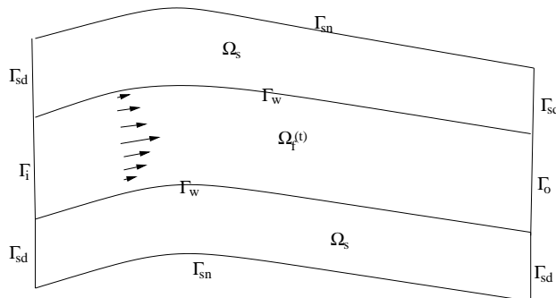
Figure 1: \Omega_0 is the reference configuration of the fluid domain and \Omega_f(t) represents the moving fluid domain at time t ; \Omega_s is the structure domain in the reference (Lagrangian) configuration. \Gamma_i and \Gamma_o are the inlet and outlet boundaries, respectively, to the fluid domain. The dry boundary to the structure \Gamma_s is further subdivided into a Dirichlet portion \Gamma_{sd} at inlets and outlets and a Neumann portion \Gamma_{sn} elsewhere. \Gamma_w is the wet fluid-structure interaction surface.
