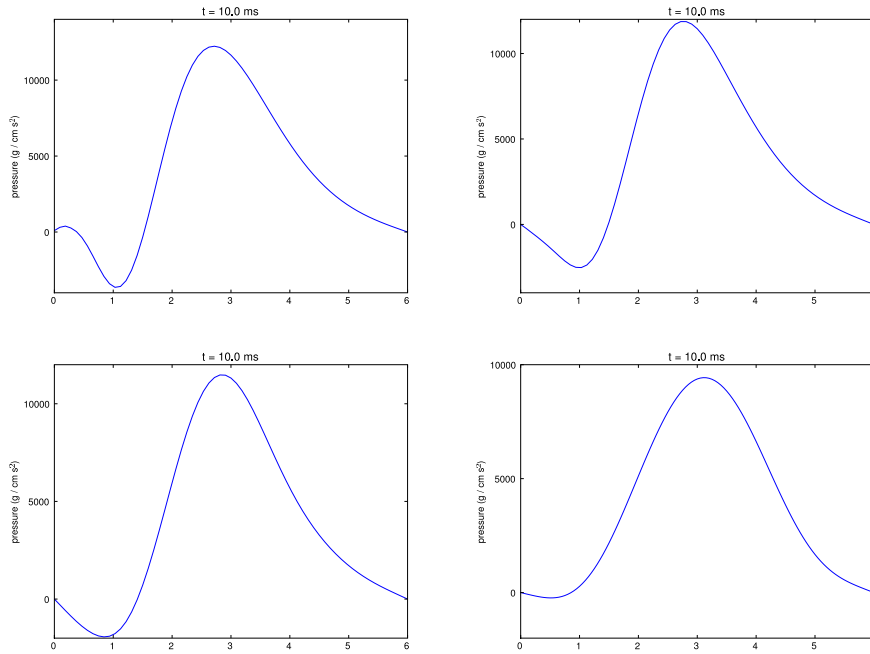
Figure 10: The pressure pulse in the straight tube problem, at 10 ms, for various values of the Young's modulus E . At top left, E = 7.5 \cdot 10^3 \text{ kg/m} \cdot \text{s}^2 , at top right E = 3.0 \cdot 10^4 \text{ kg/m} \cdot \text{s}^2 , at bottom left E = 7.5 \cdot 10^4 \text{ kg/m} \cdot \text{s}^2 (the physiological value used in [2]), and at bottom right E = 7.5 \cdot 10^5 \text{ kg/m} \cdot \text{s}^2 , which was used in [30]. In all cases \beta = 0.001 \text{ kg/m} \cdot \text{s} . These plots are to be compared to the bottom left plot in Figures 6 and 7. The profiles are somewhat different for different E but are qualitatively similar.
