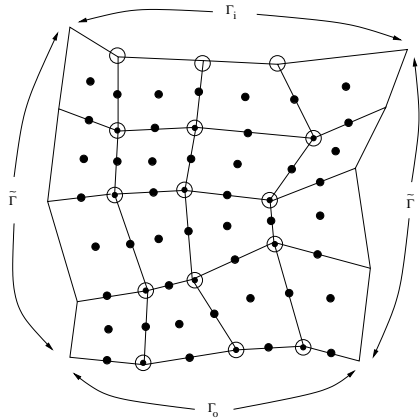
Figure 4: Boundary conditions for a (fluid-only) subdomain problem. ( \bullet ) represents a fluid velocity degree of freedom and ( \circ ) is fluid pressure. The top and bottom boundaries are physical boundaries, where physical Dirichlet ( \Gamma_i ) or Neumann ( \Gamma_o ) conditions are applied; the left and right boundaries are subdomain boundaries ( \tilde{\Gamma} ) not corresponding to physical boundaries, where for the subdomain preconditioner non-physical Dirichlet conditions are applied.
