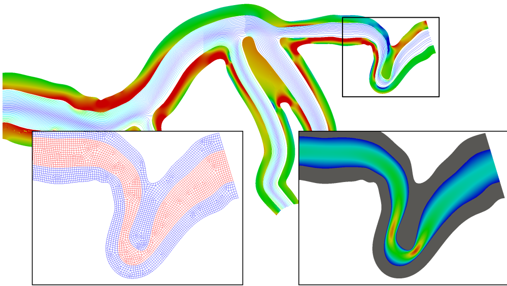
Figure 12: A portion of our branched computational model. In the main image, the structure is colored by pressure and fluid streamlines are colored by vorticity. In the left inset is a detail of the quadrilateral mesh; in the right inset is a detail of the fluid velocity, both insets representing a magnification of the marked portion.
