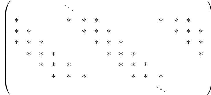
Figure 5: Nonzero block structure of the Jacobian matrix. The size of the blocks varies, but is no larger than 40 and usually no smaller than 17.
