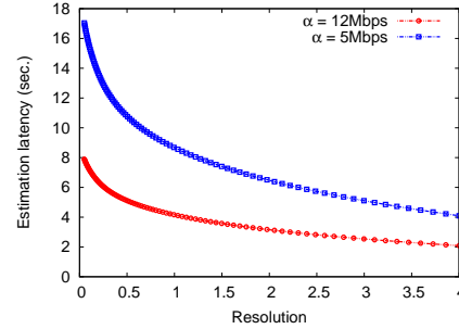
Figure 15: Measurement latency at different resolutions.
