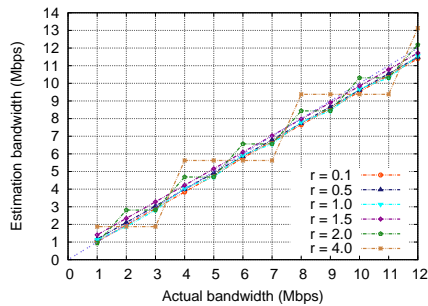
Figure 8: Bandwidth estimation.
