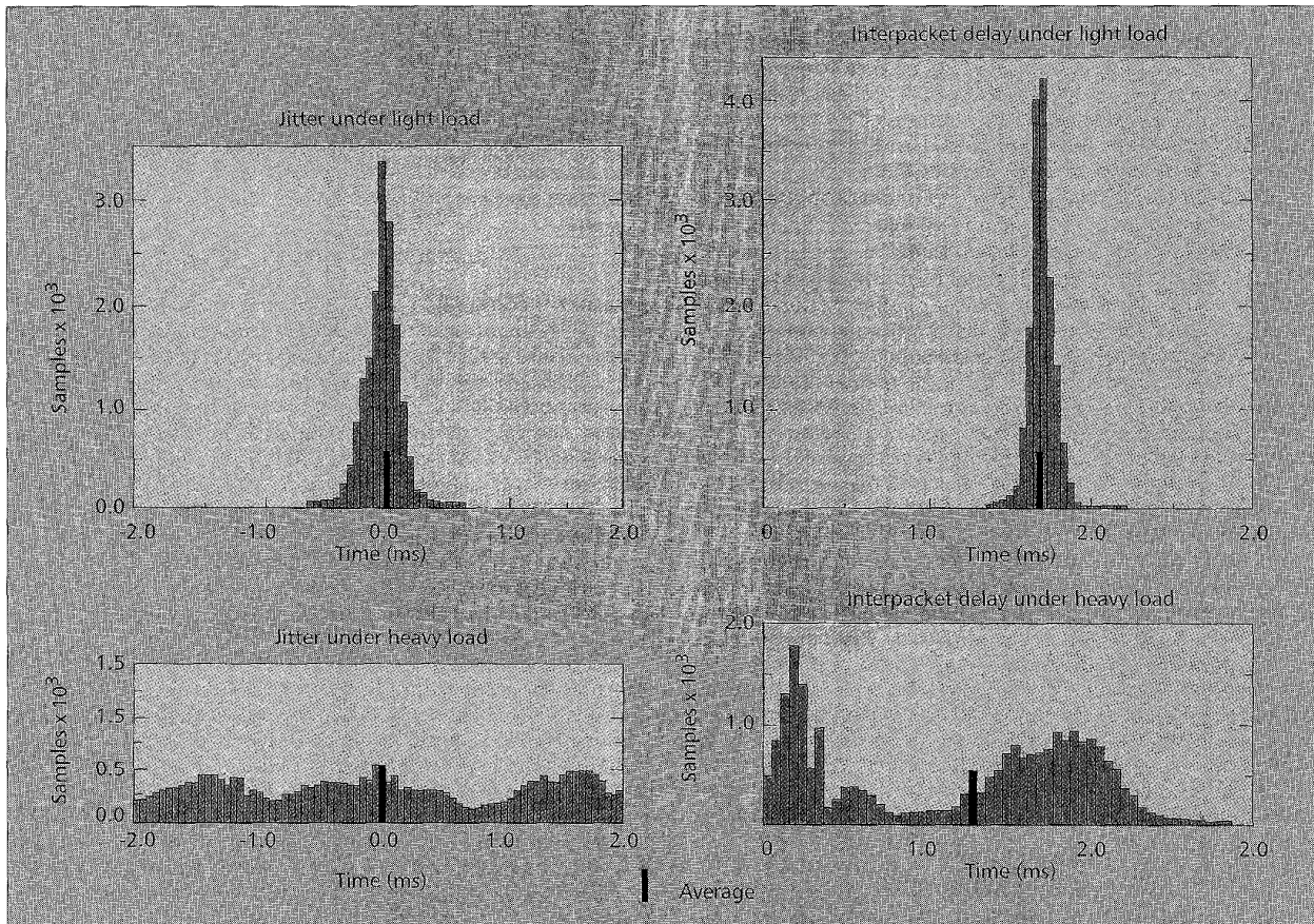
■ Figure 14. Example jitter and interpacket delay histograms.
