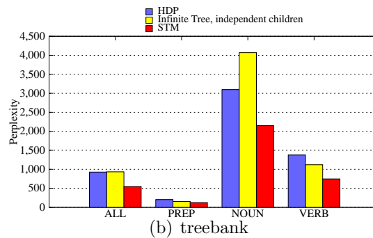
Figure 5.8: After fitting three models on synthetic data, the syntactic topic model has better (lower) perplexity on all word classes except for adjectives. HDP is better able to capture document-level patterns of adjectives. The infinite tree captures prepositions best, which have no cross-document variation. On real data 5.8(b), the syntactic topic model was able to combine the strengths of the infinite tree on functional categories like prepositions with the strengths of the HDP on content categories like nouns to attain lower overall perplexity.
