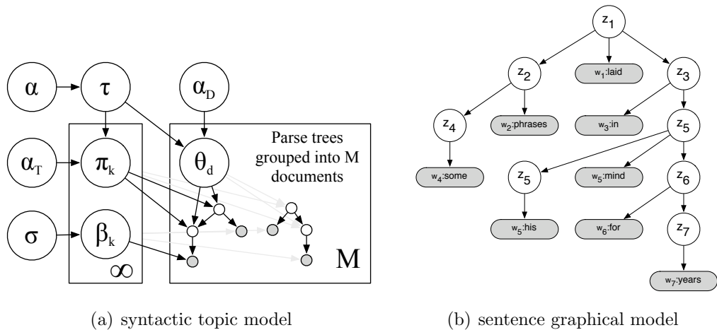
Figure 5.3: In this graphical model depiction of the syntactic topic model, the dependency parse representation of FTIC in Figure 5.1(b) are grouped into documents, as in LDA in 5.1(a). For each of the words in the sentence, the topics weights of a document \theta and the parent’s topic transition \pi together choose the topic. (For clarity, some of the sentence node dependencies have been grayed out.) An example of the structure of a sentence is on the right, as demonstrated by an automatic parse of the sentence “Some phrases laid in his mind for years.” The STM assumes that the tree structure and words are given, but the latent topics \mathbf{z} are not.
